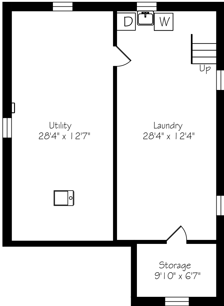
Lower Level 918 Square Feet
